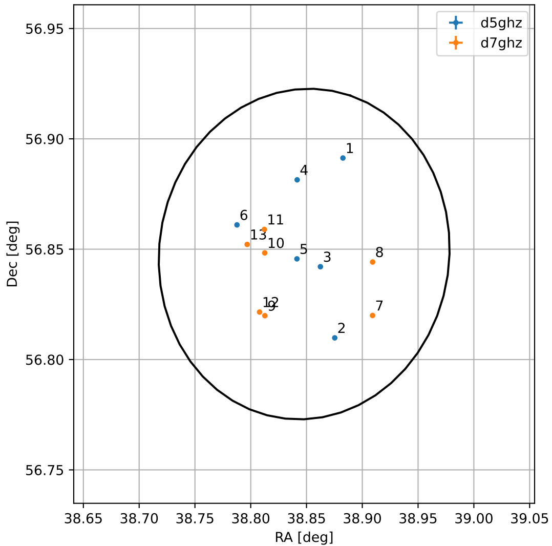
4FGL J0235.3+5650
