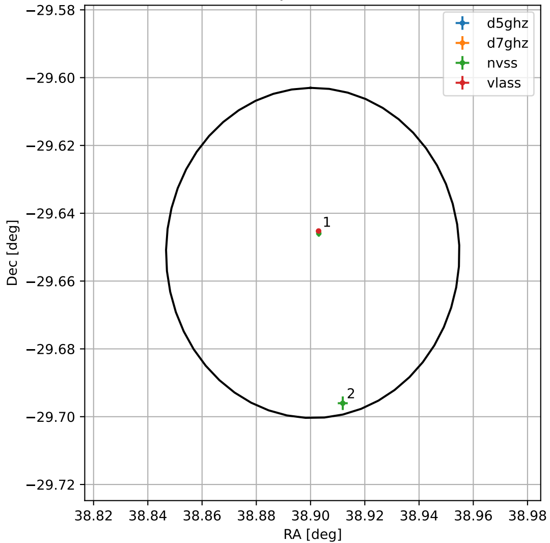
4FGL J0235.6-2939
