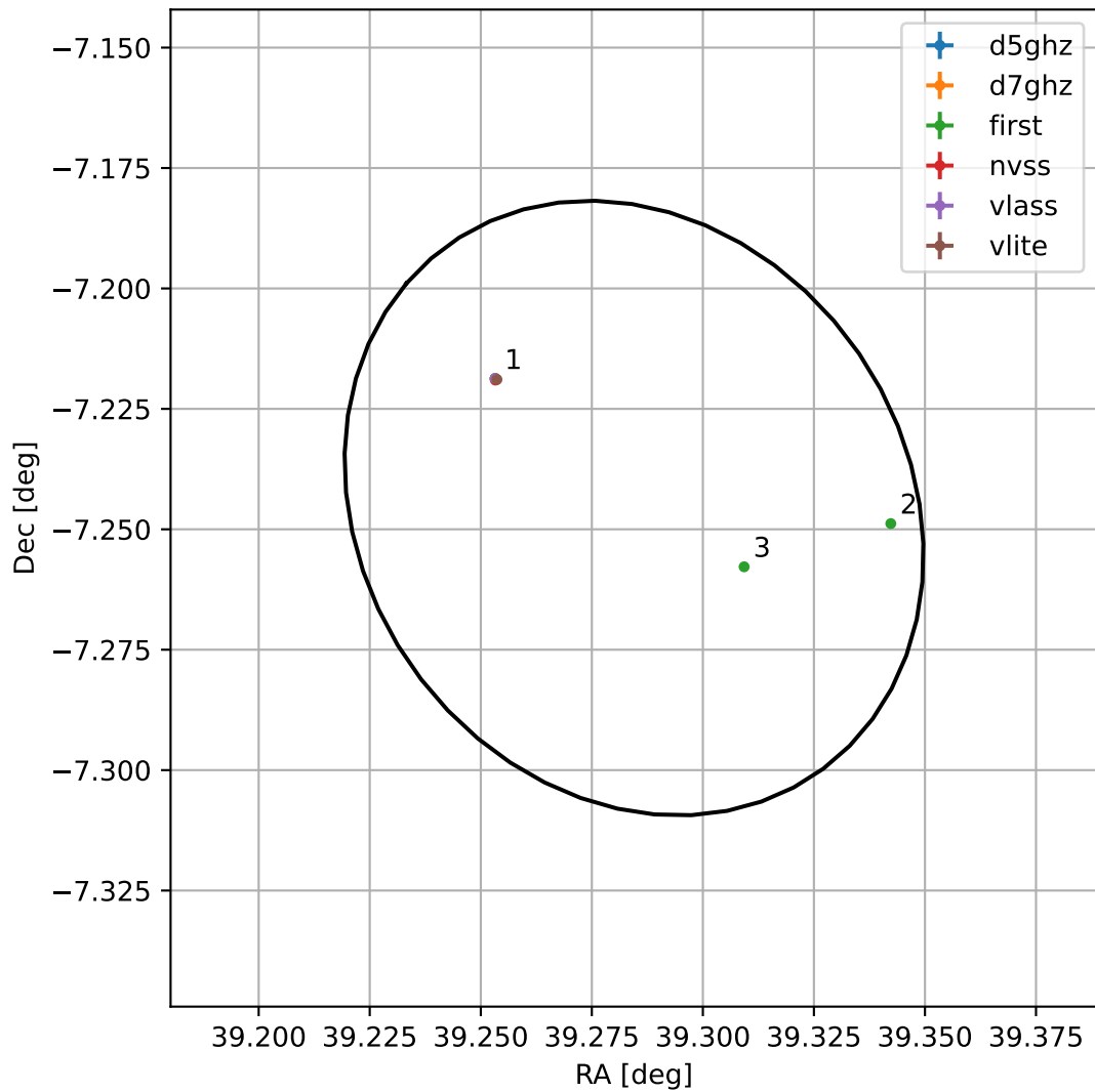
4FGL J0237.1-0714
