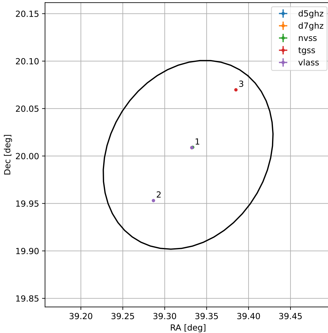
4FGL J0237.3+2000
