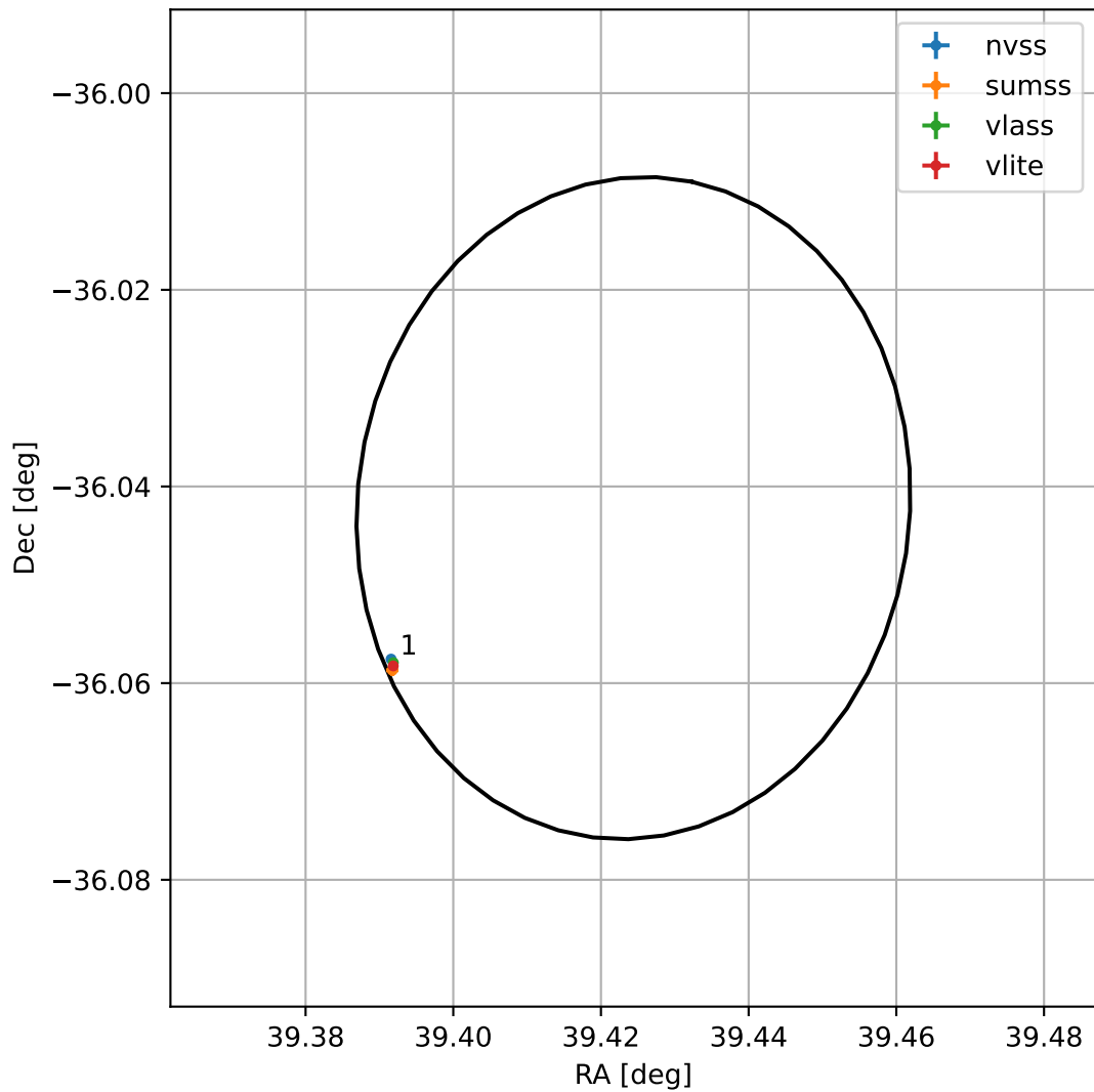
4FGL J0237.6-3602
