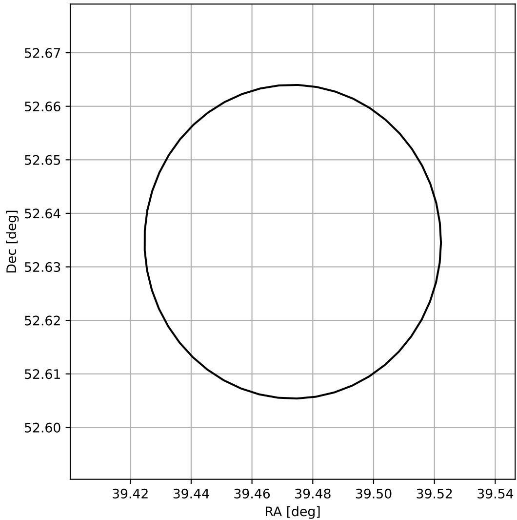
4FGL J0237.8+5238
