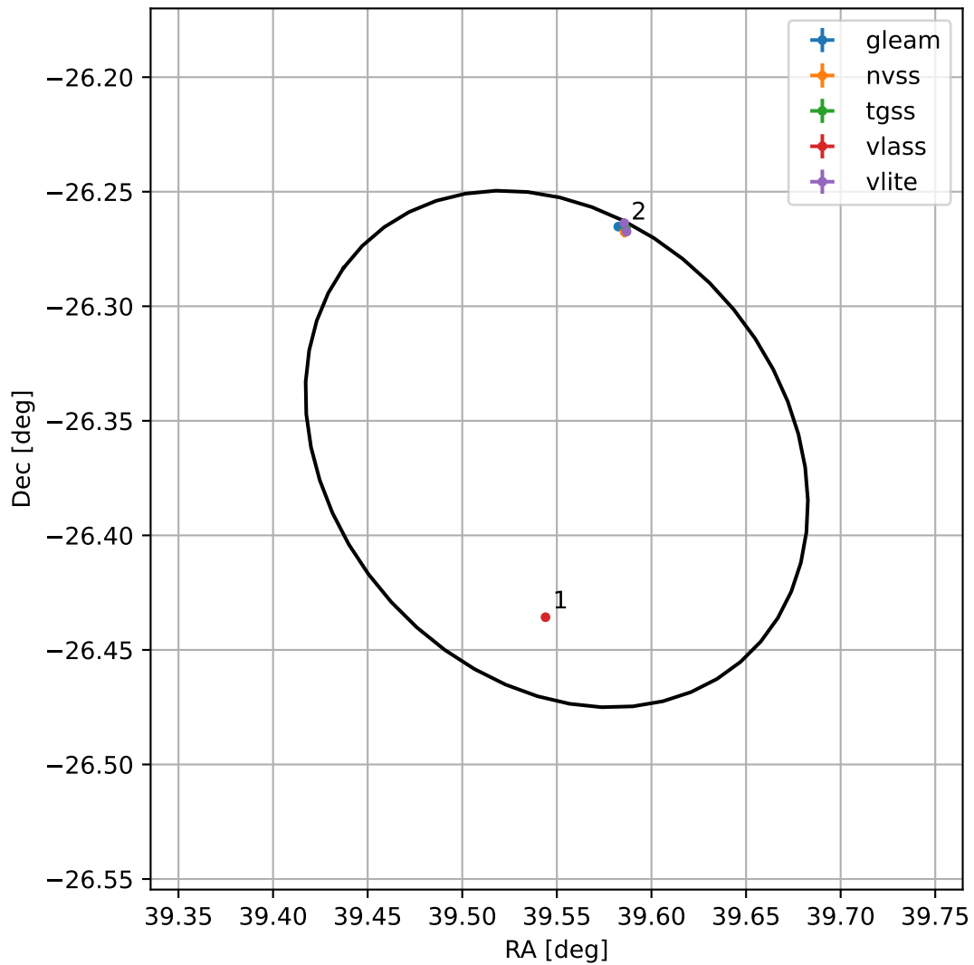
4FGL J0238.1-2621
