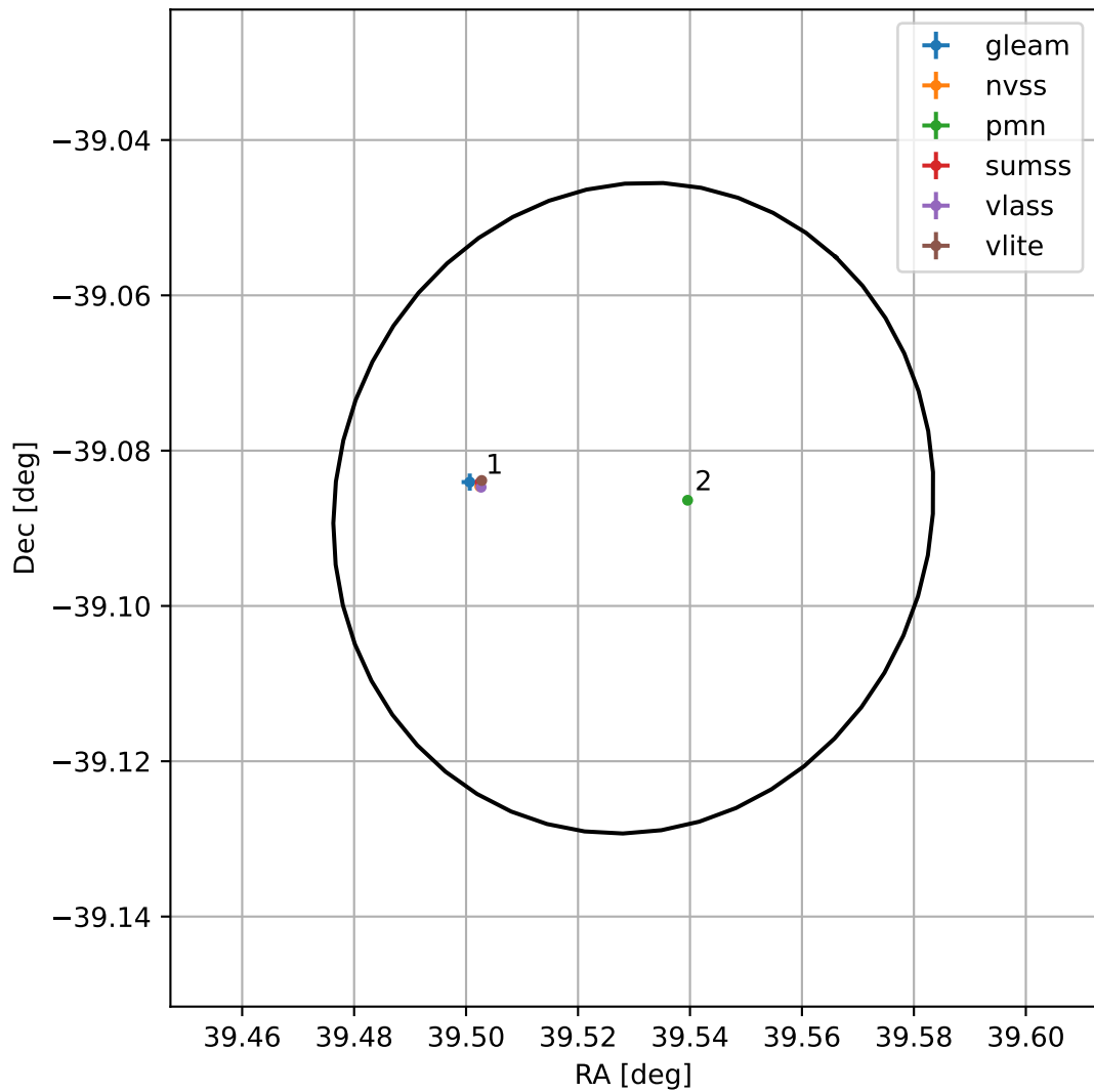
4FGL J0238.1-3905
