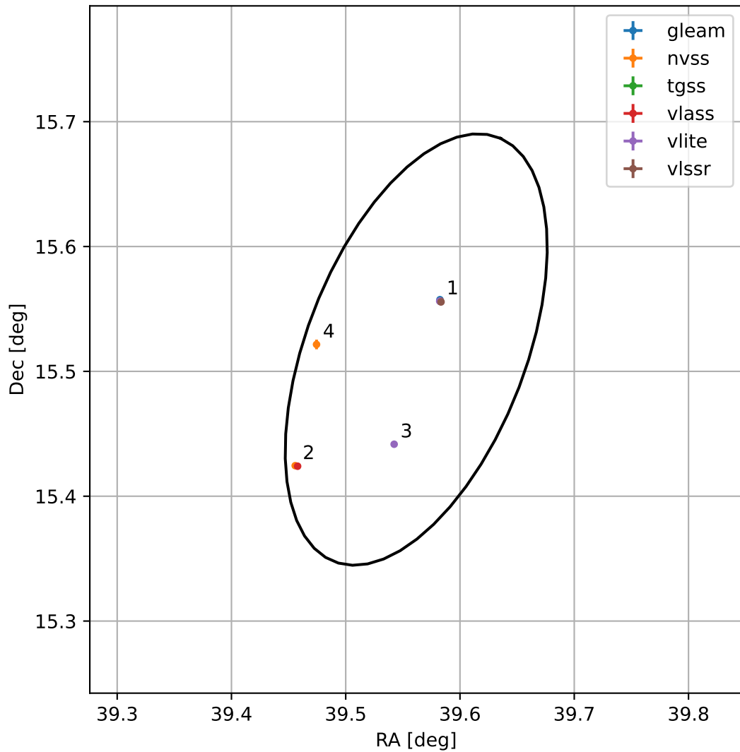
4FGL J0238.2+1531
