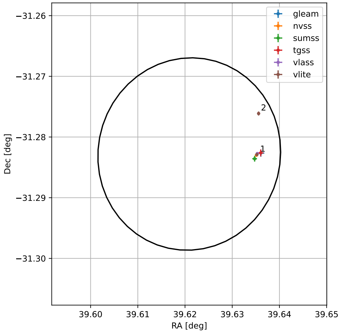
4FGL J0238.4-3116
