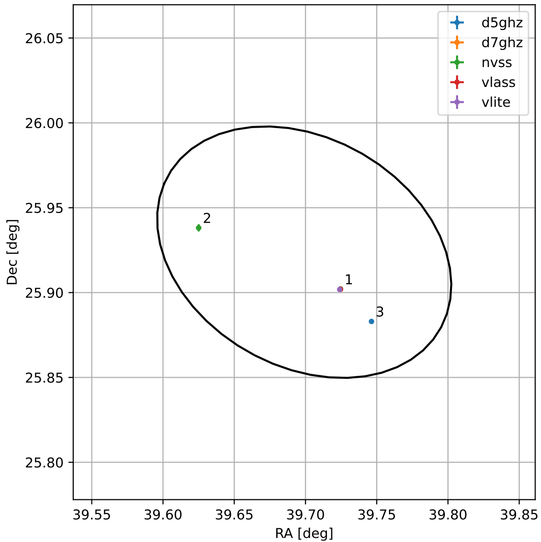
4FGL J0238.7+2555
