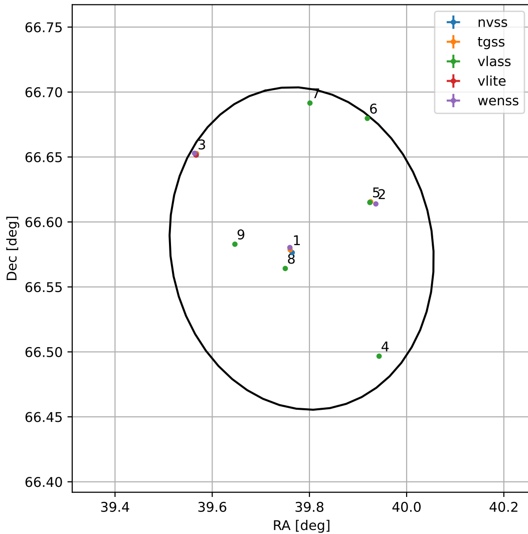
4FGL J0239.1+6634
