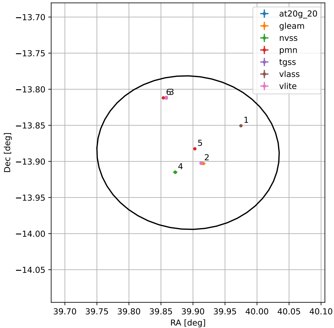
4FGL J0239.5-1353
