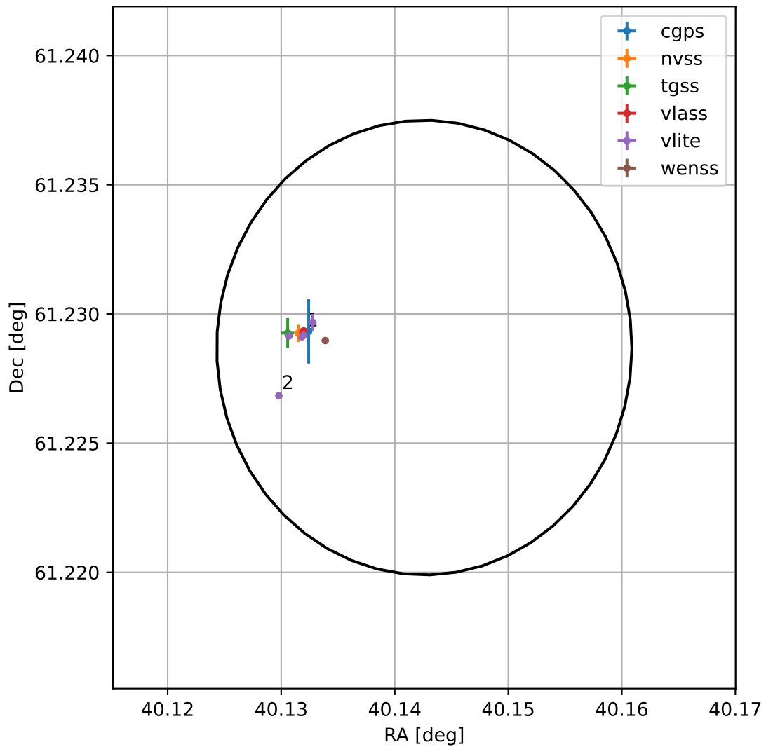
4FGL J0240.5+6113
