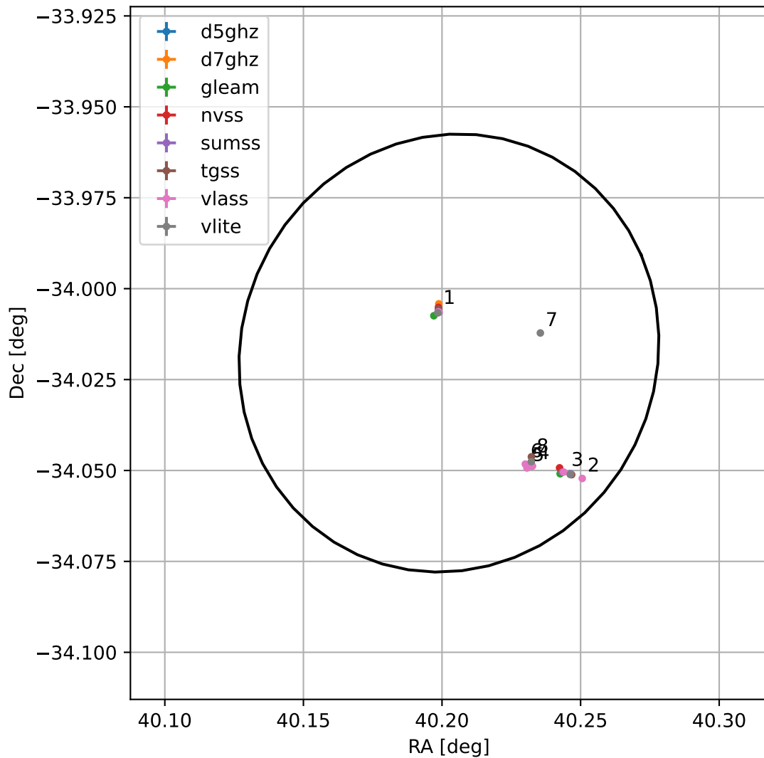
4FGL J0240.8-3401
