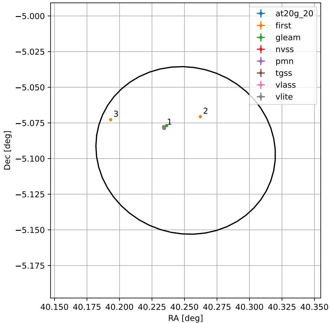
4FGL J0241.0-0505
