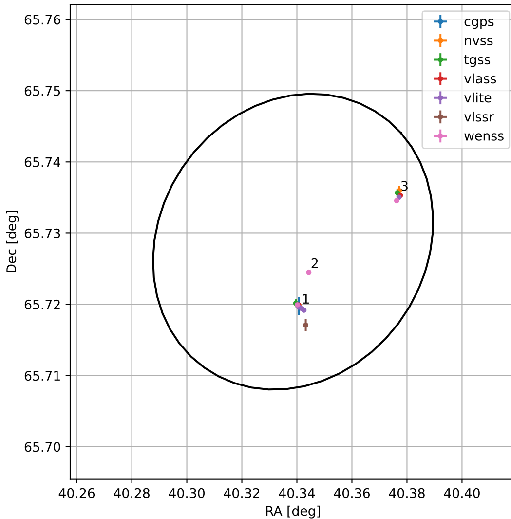
4FGL J0241.3+6543
