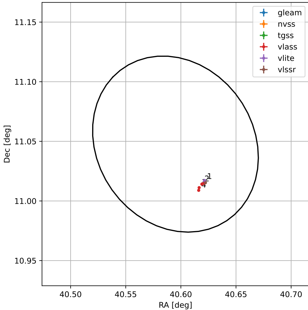
4FGL J0242.3+1102
