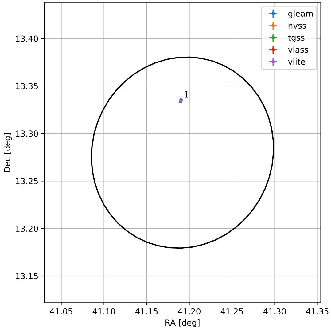
4FGL J0244.7+1316
