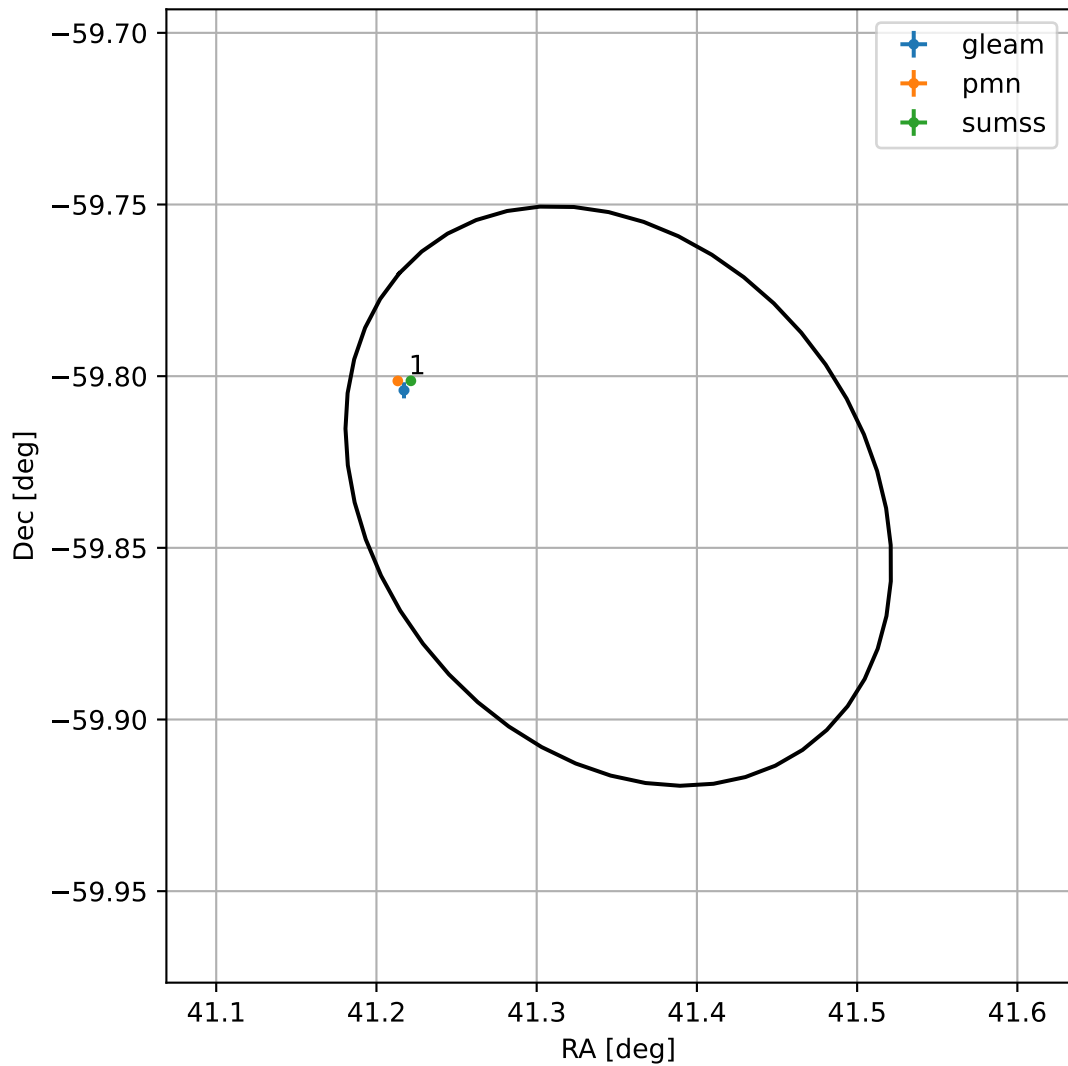
4FGL J0245.4-5950
