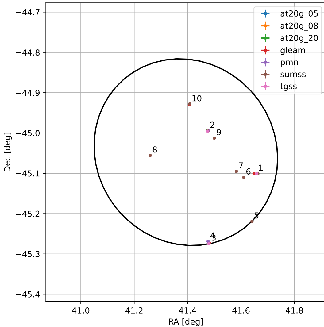
4FGL J0245.5-4502
