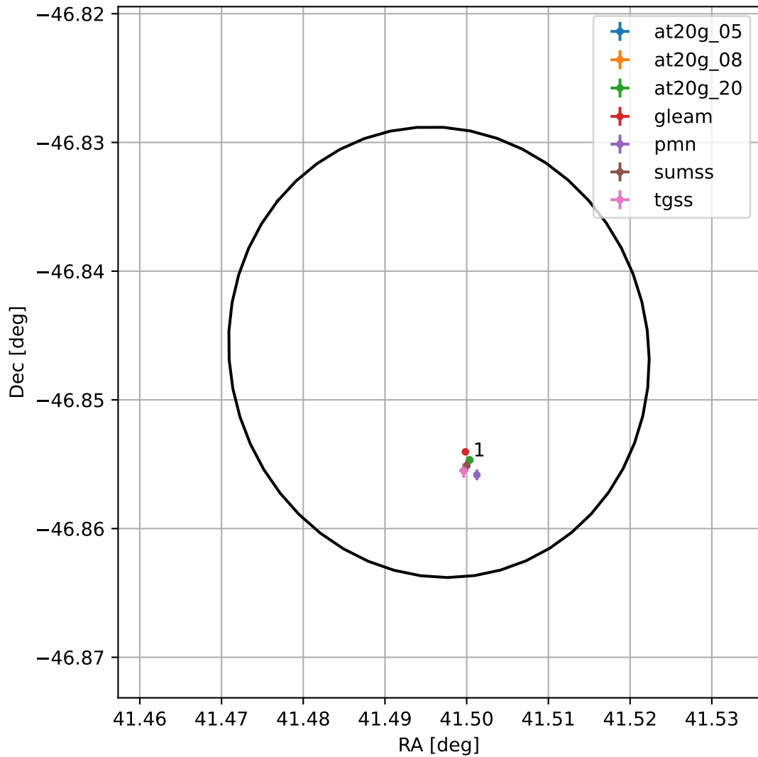
4FGL J0245.9-4650
