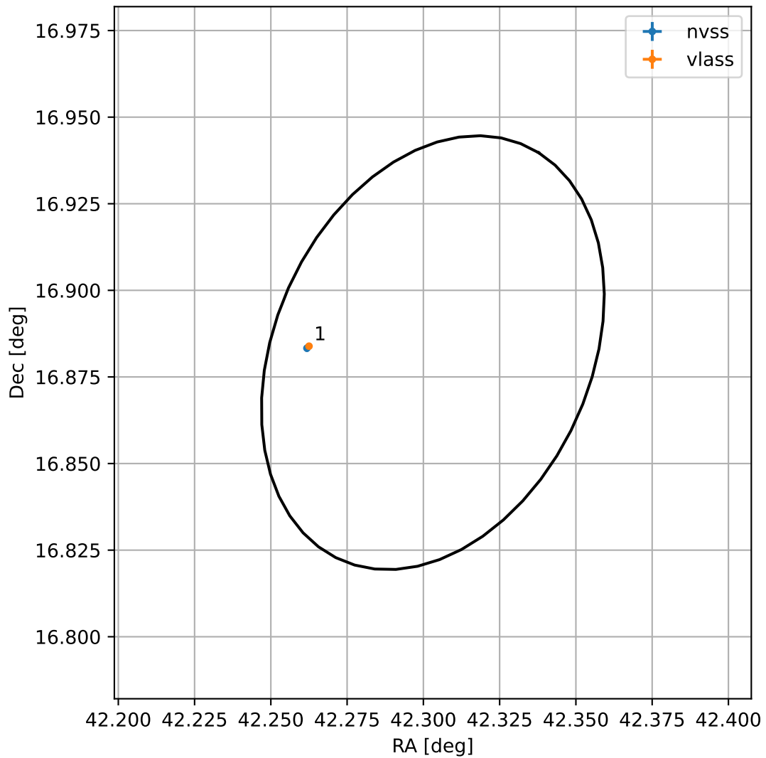
4FGL J0249.2+1652
