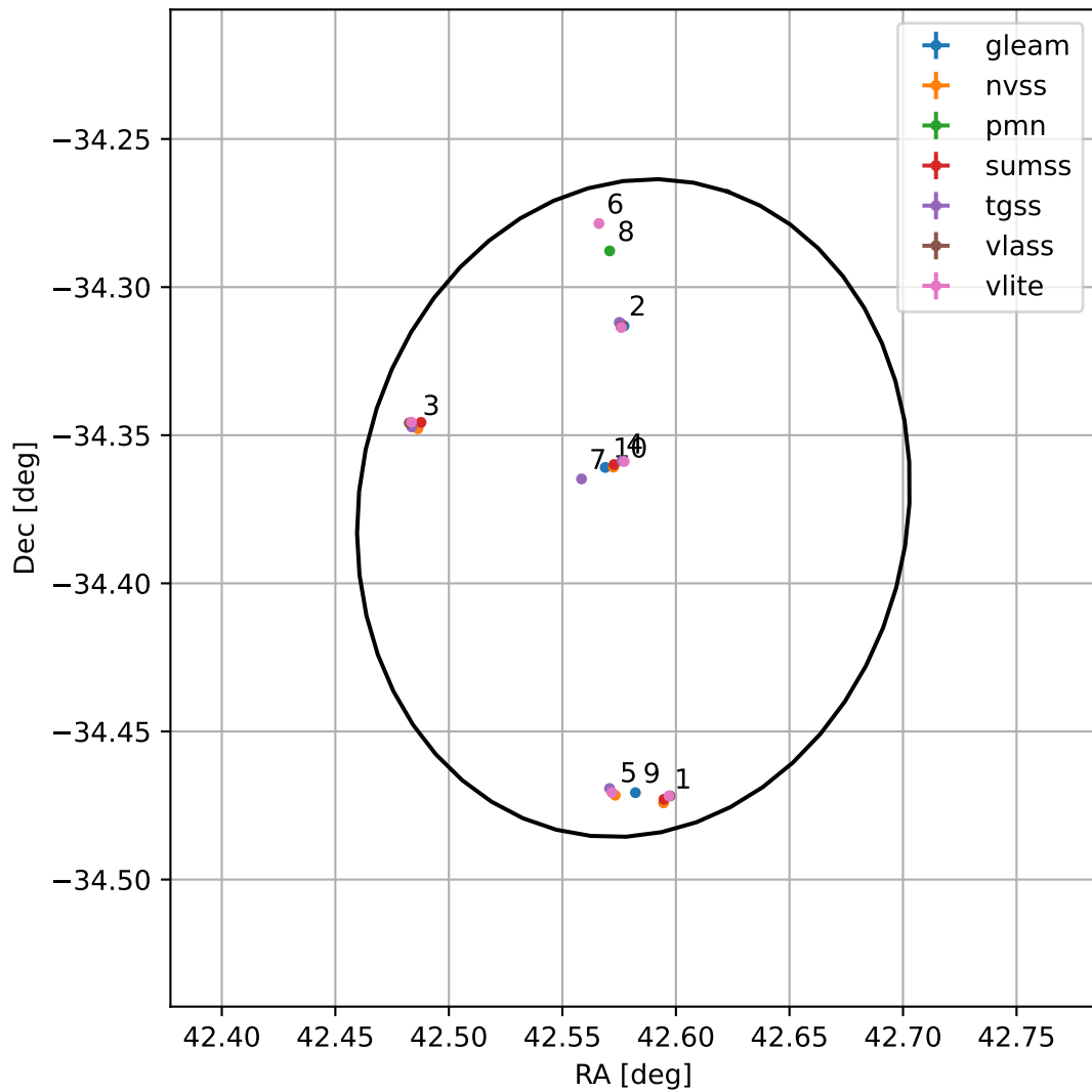
4FGL J0250.3-3422
