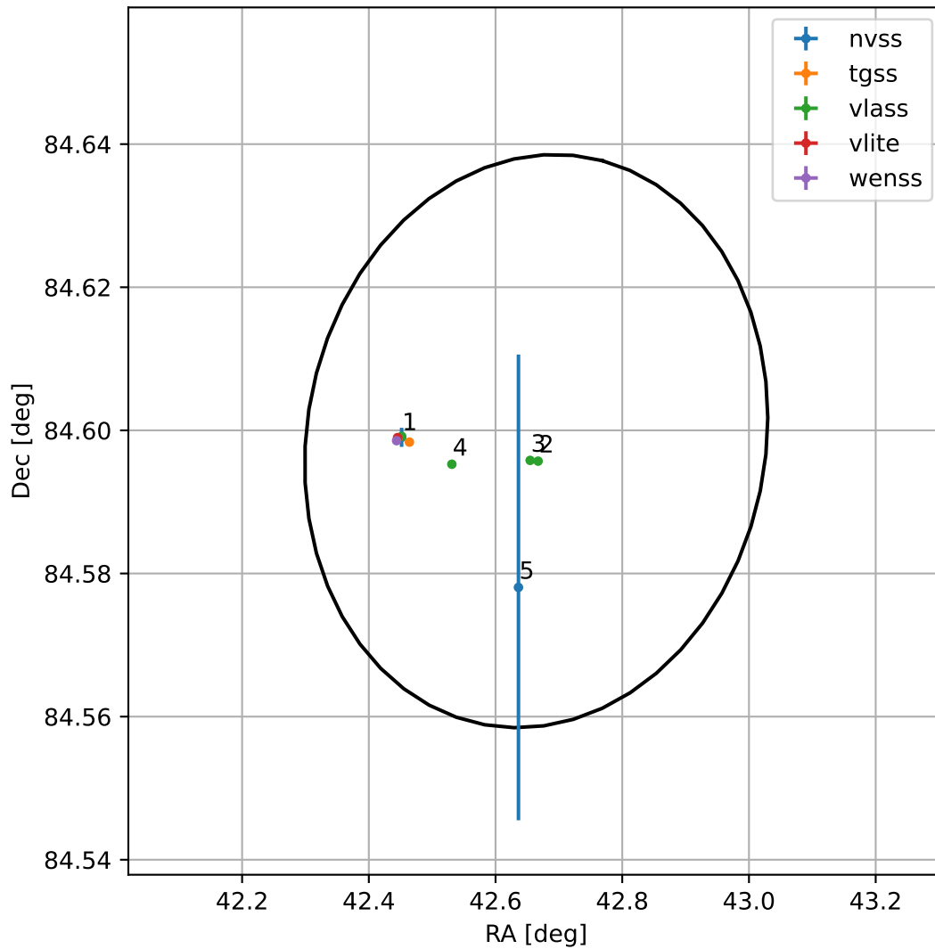
4FGL J0250.6+8435
