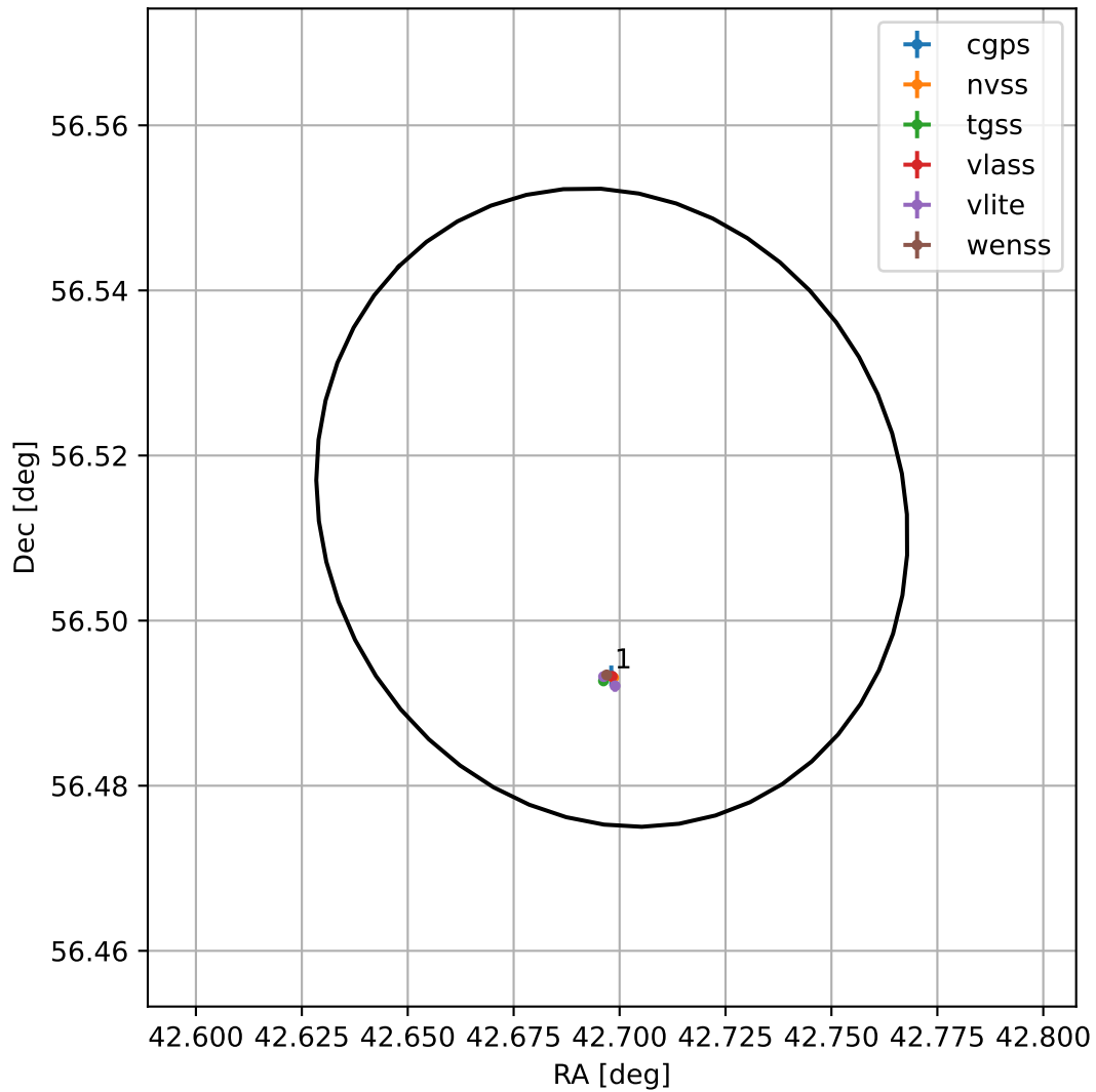
4FGL J0250.7+5630
