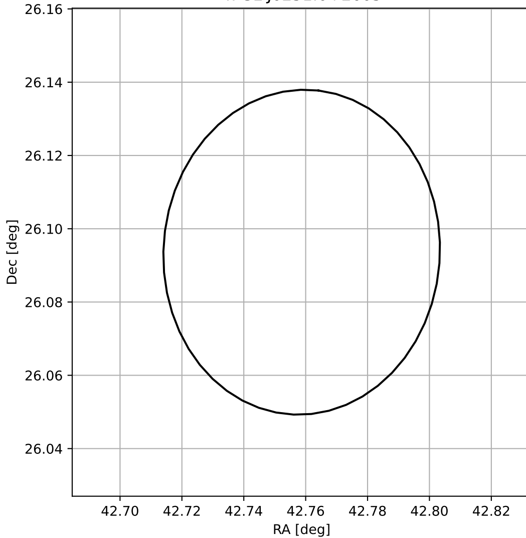
4FGL J0251.0+2605
