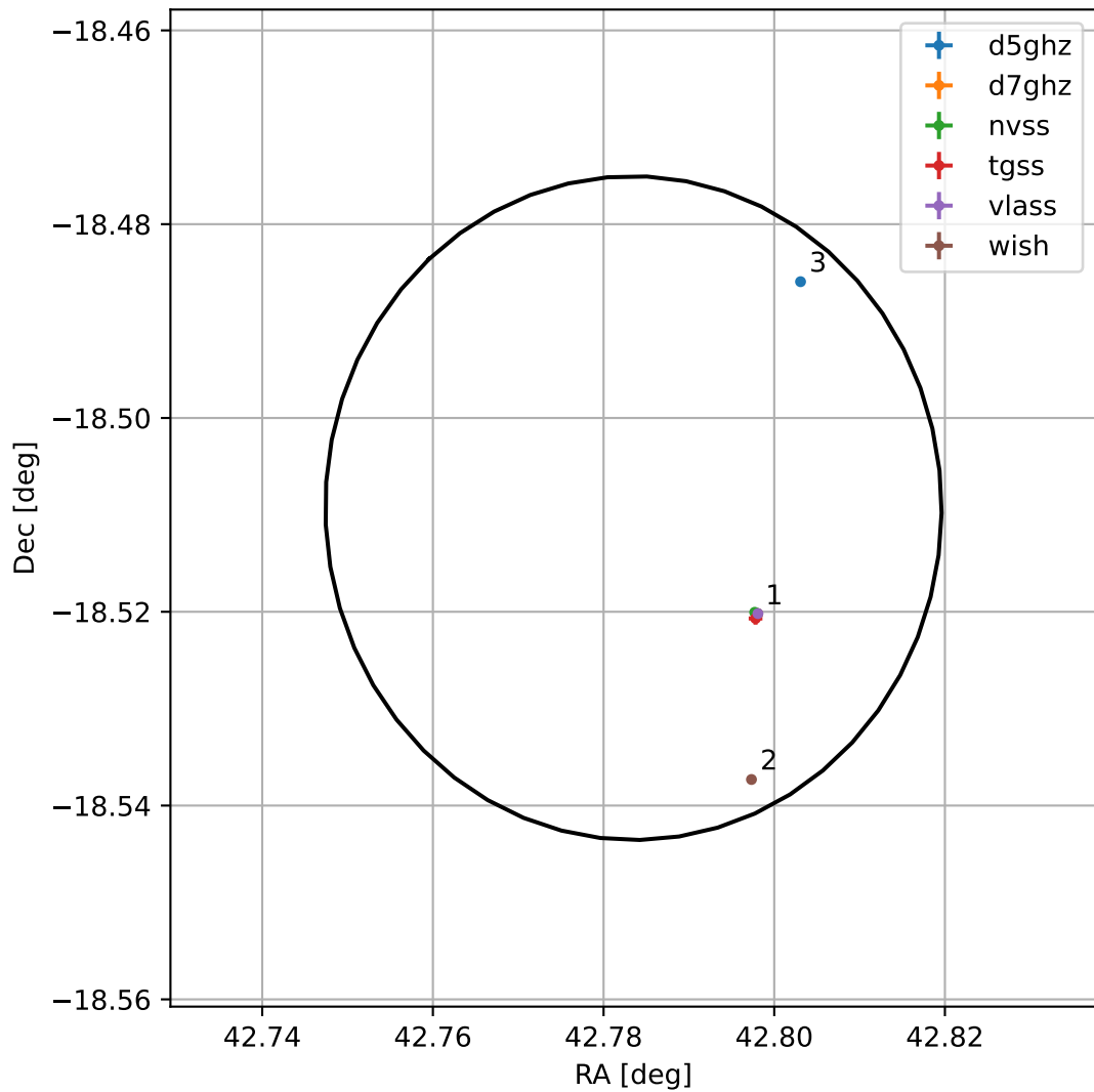
4FGL J0251.1-1830
