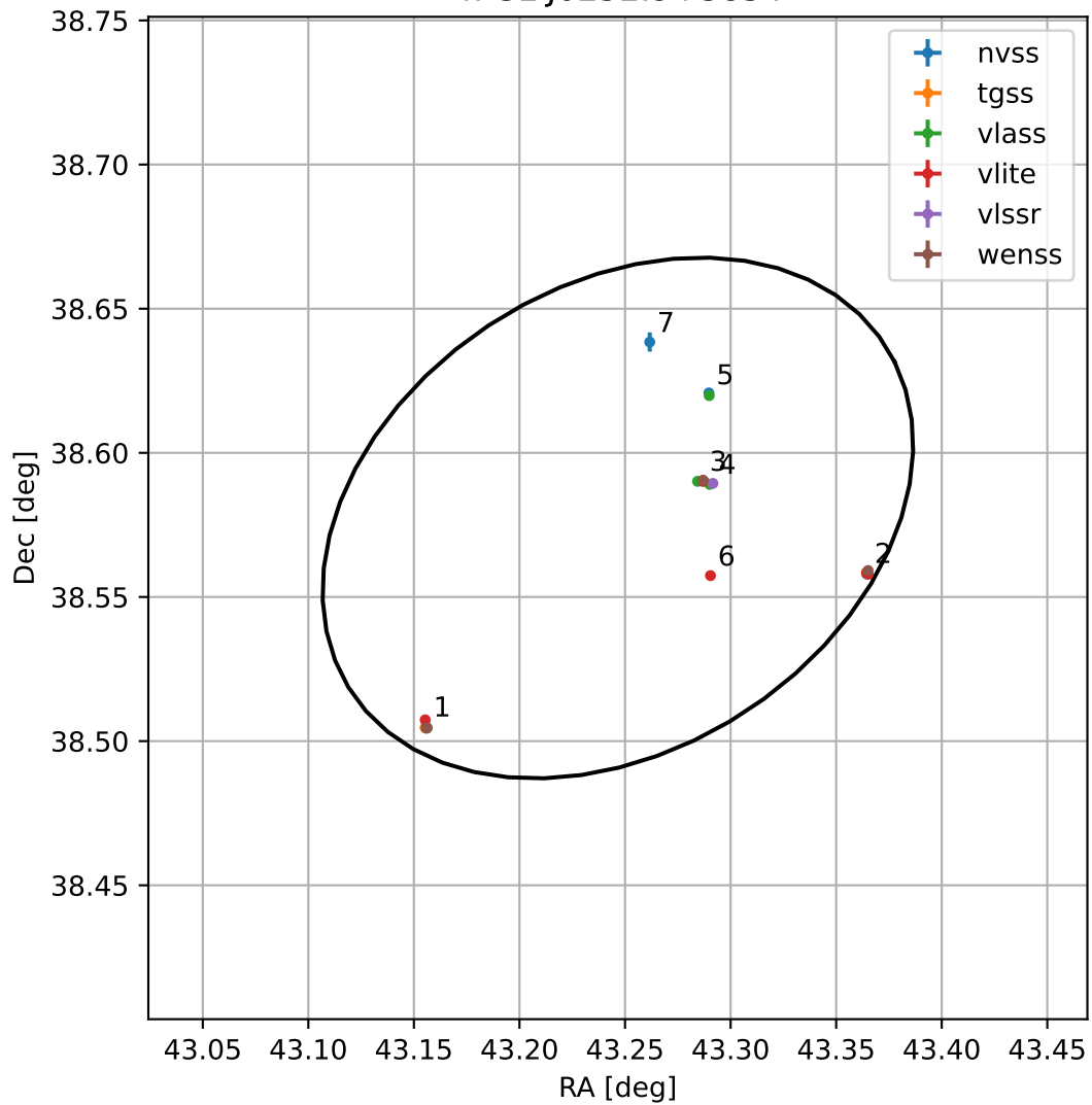
4FGL J0252.9+3834
