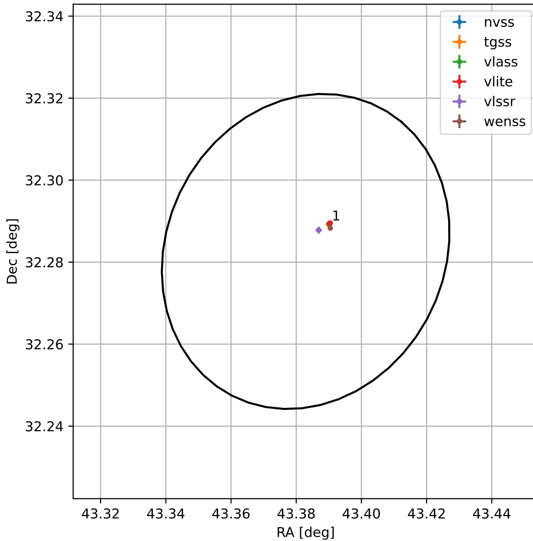
4FGL J0253.5+3216
