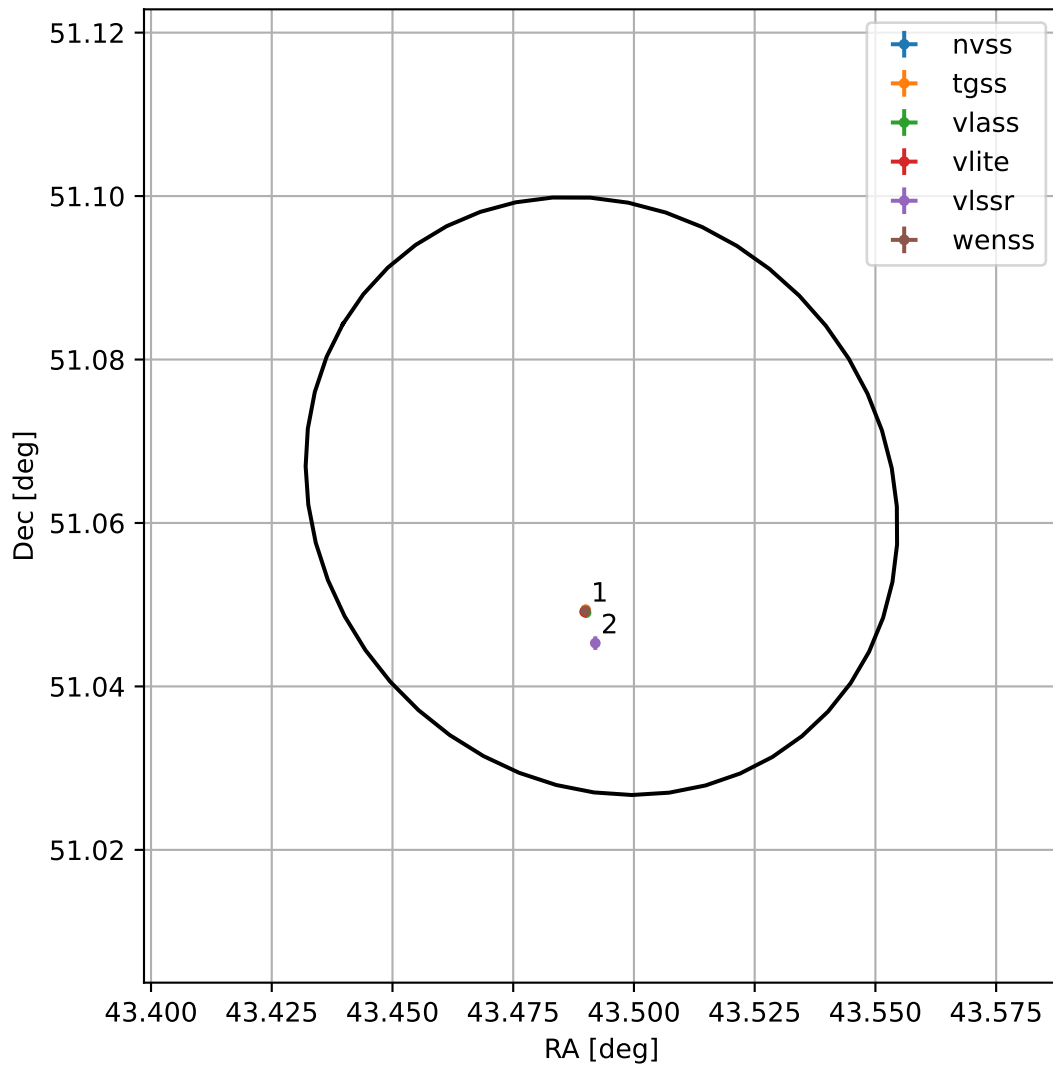
4FGL J0253.9+5103
