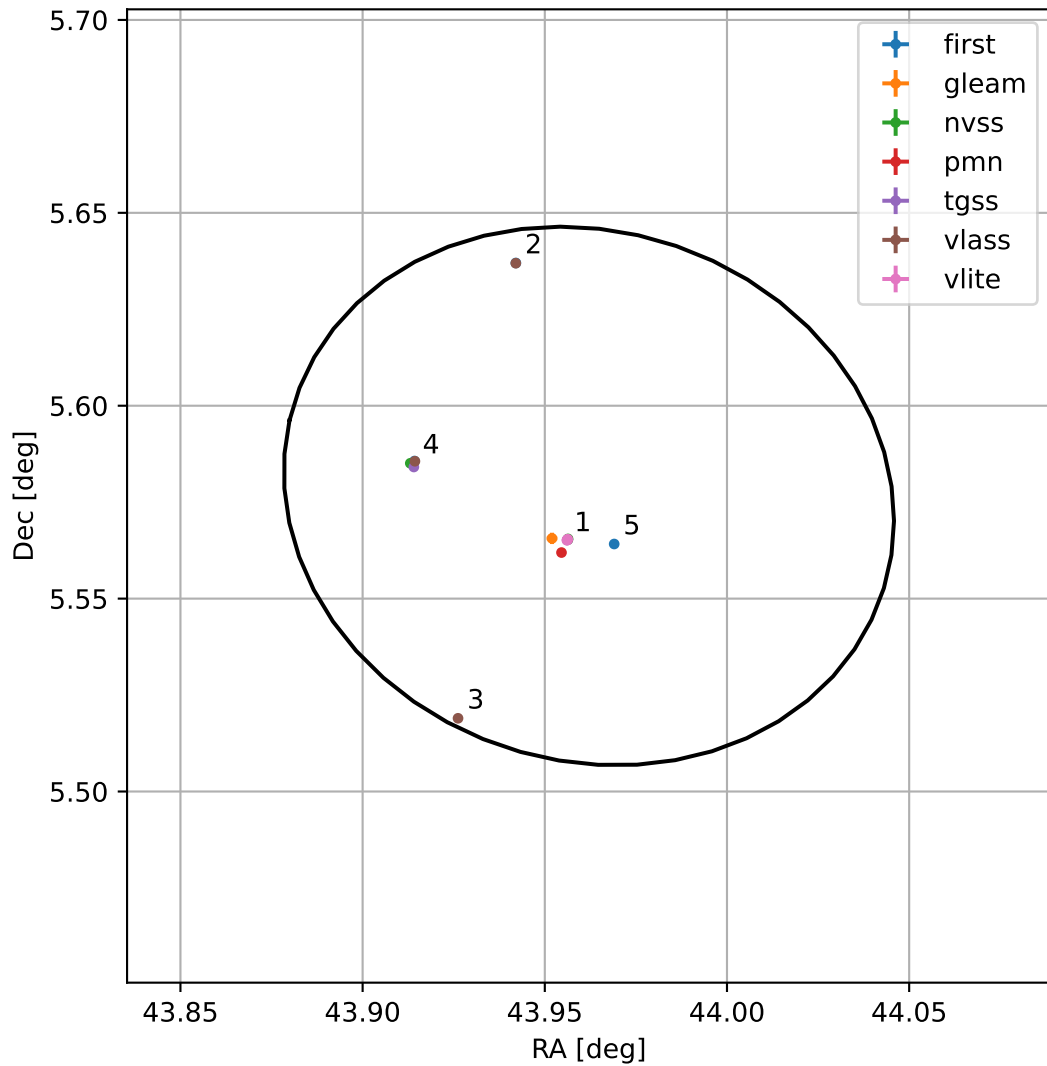
4FGL J0255.8+0534
