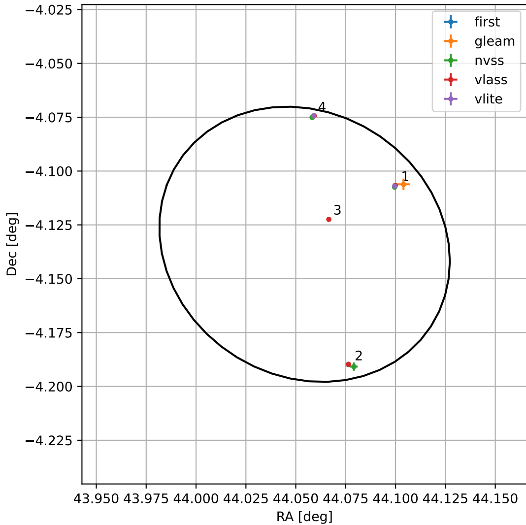
4FGL J0256.2-0408
