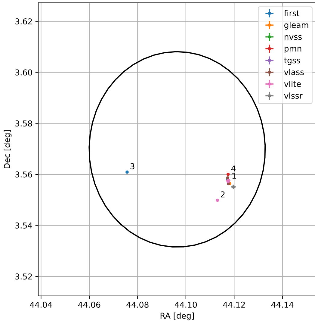
4FGL J0256.3+0334
