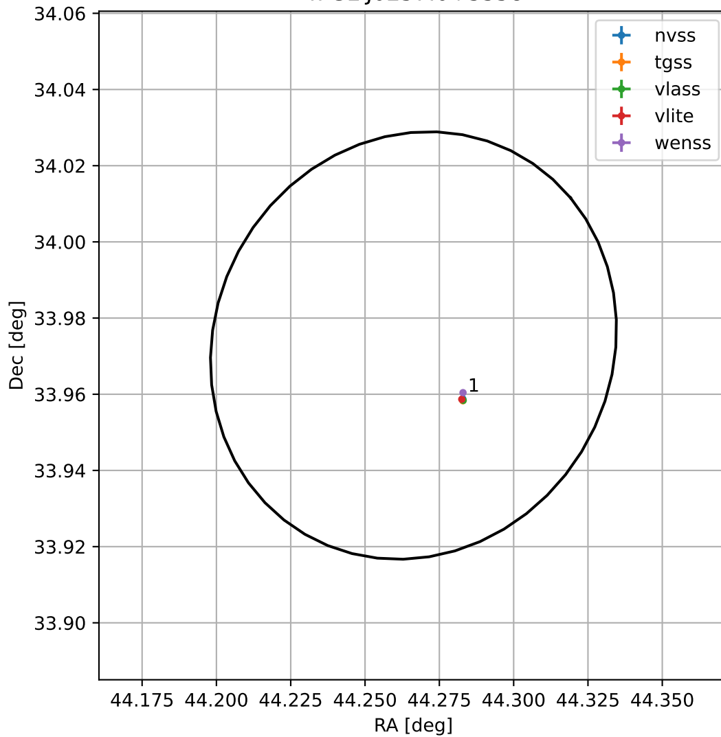
4FGL J0257.0+3358
