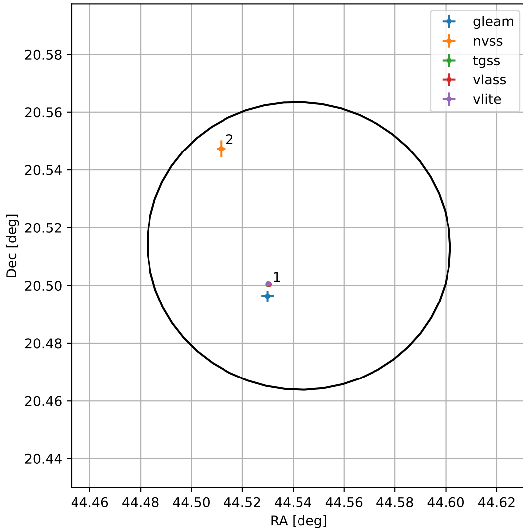
4FGL J0258.1+2030
