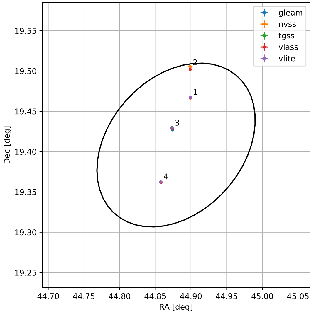
4FGL J0259.5+1924
