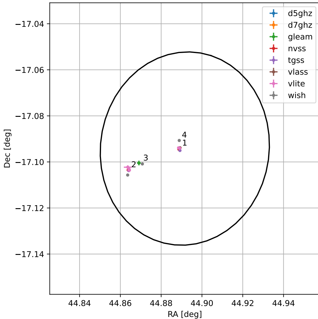
4FGL J0259.5-1705
