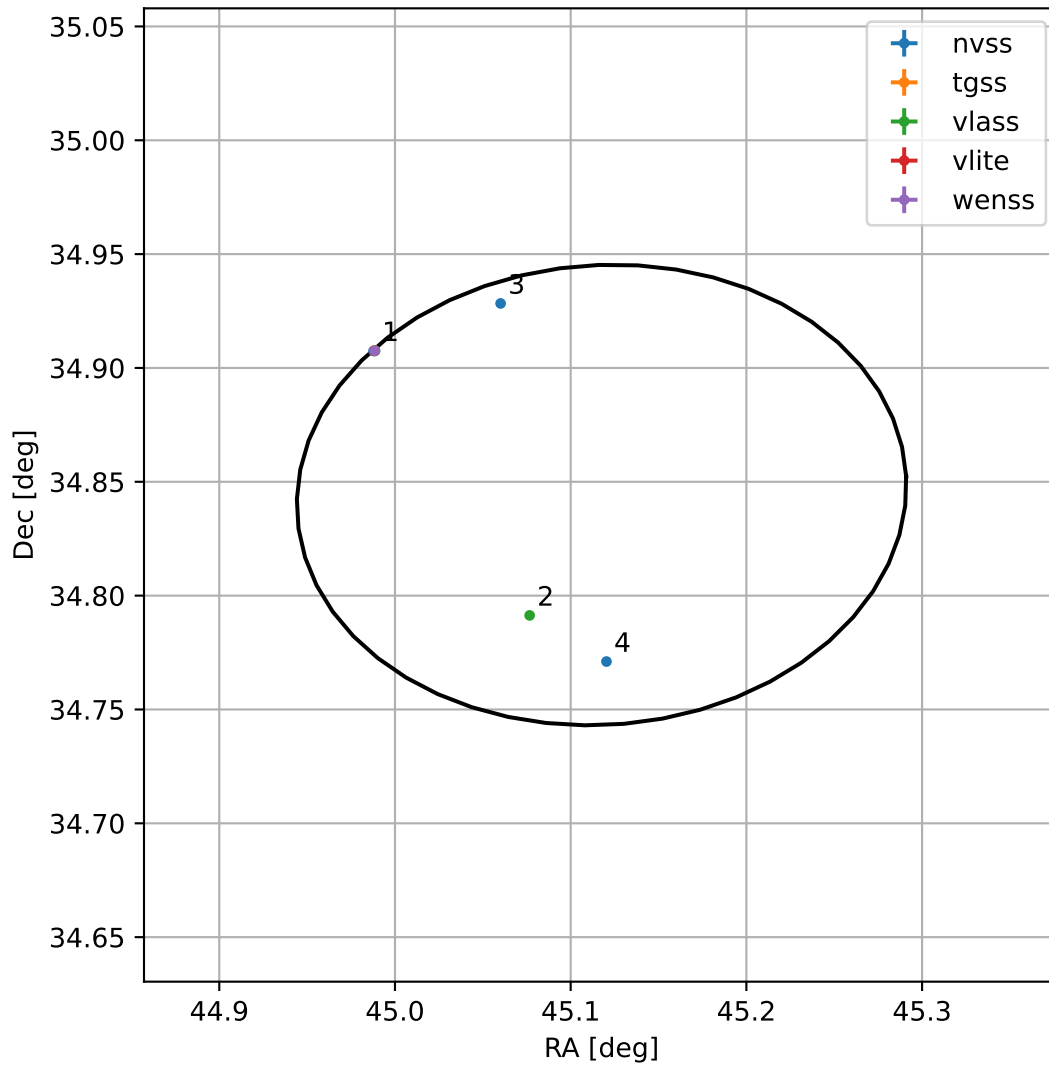
4FGL J0300.4+3450
