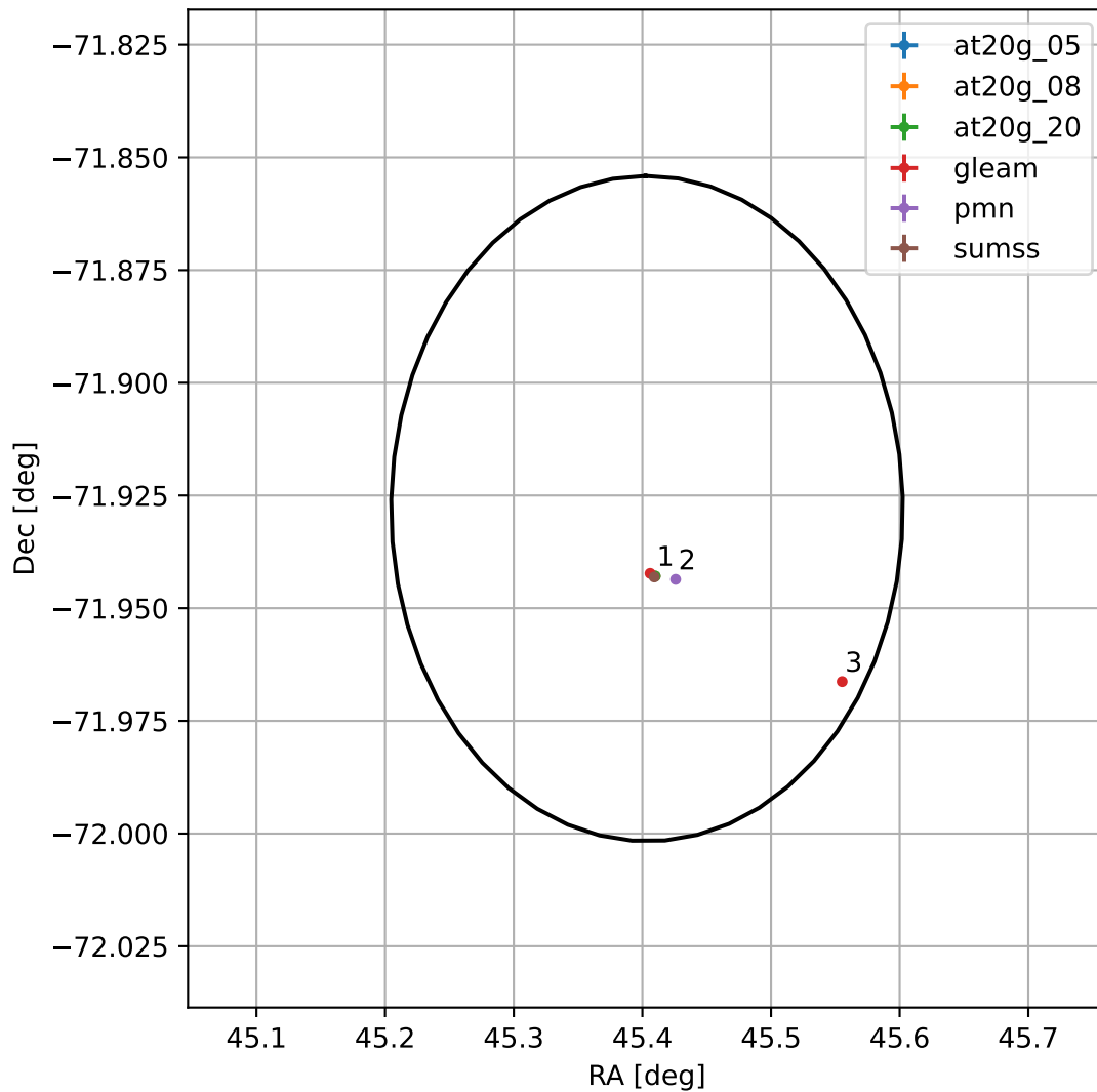
4FGL J0301.6-7155
