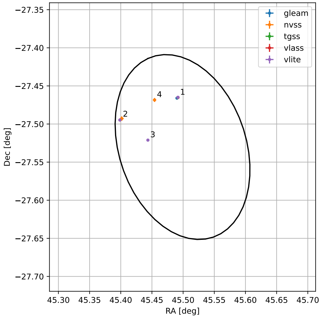
4FGL J0301.9-2731
