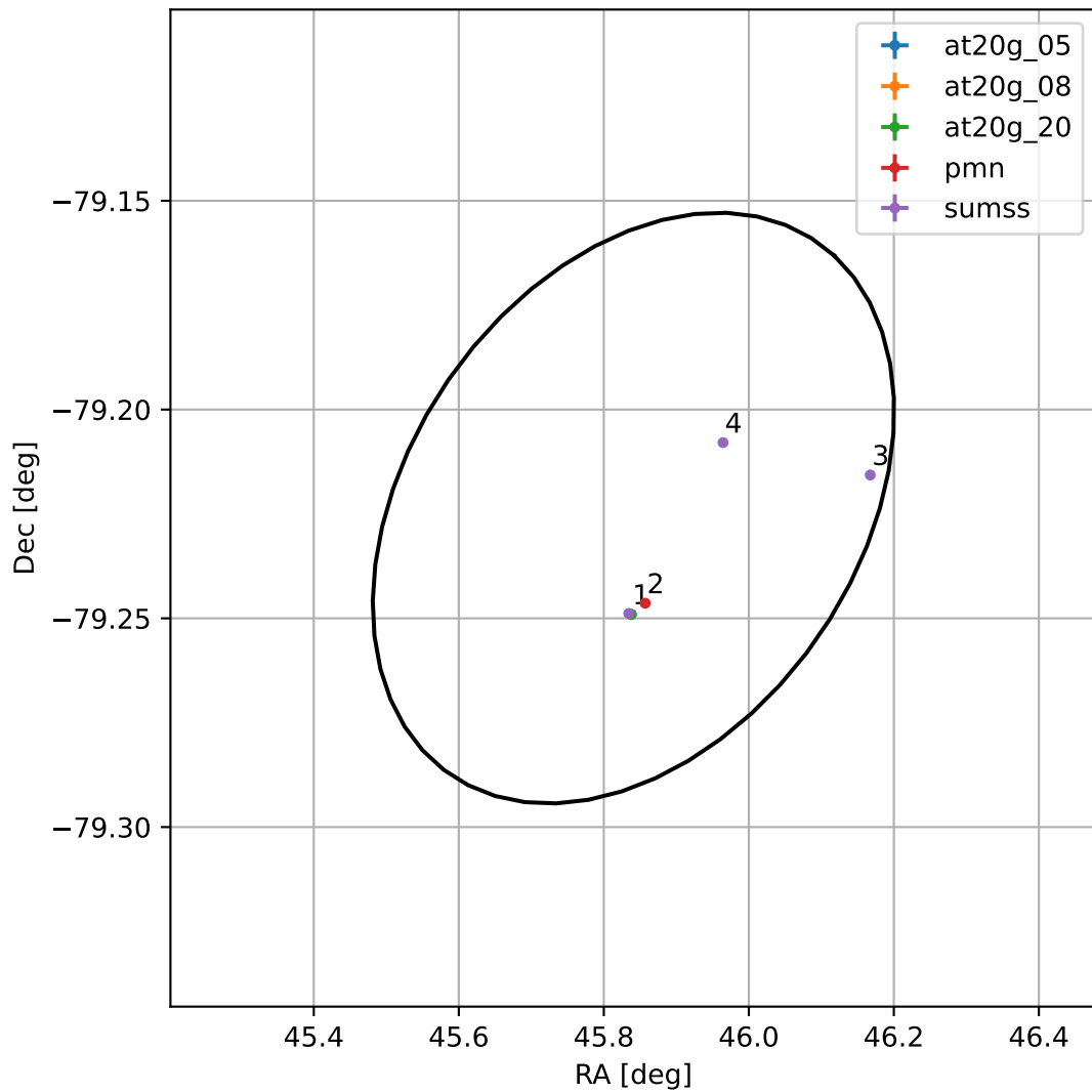
4FGL J0303.3-7913
