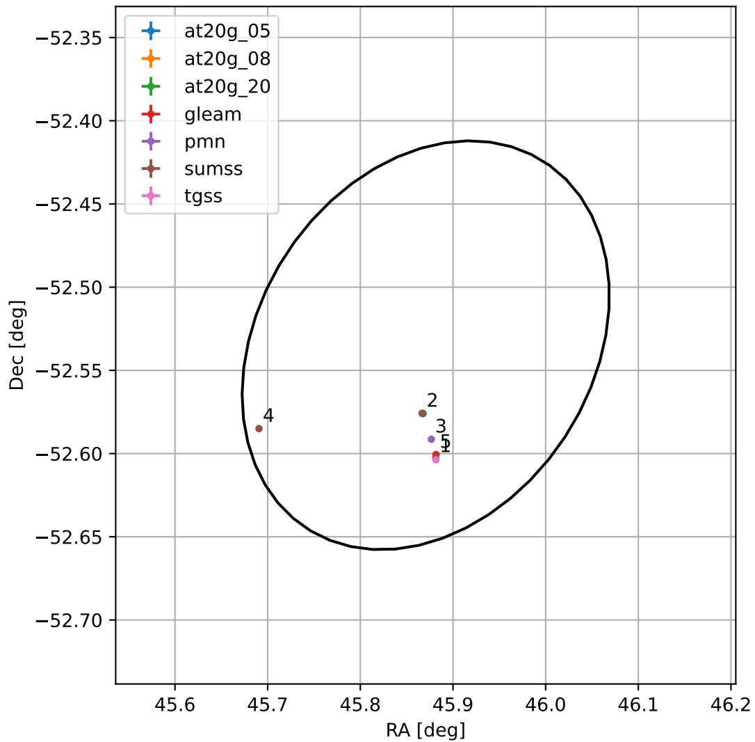
4FGL J0303.4-5232
