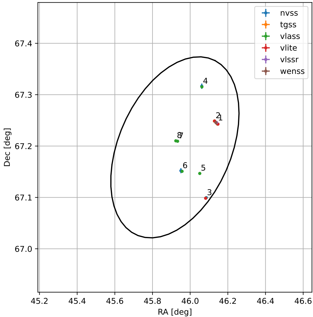
4FGL J0303.6+6711
