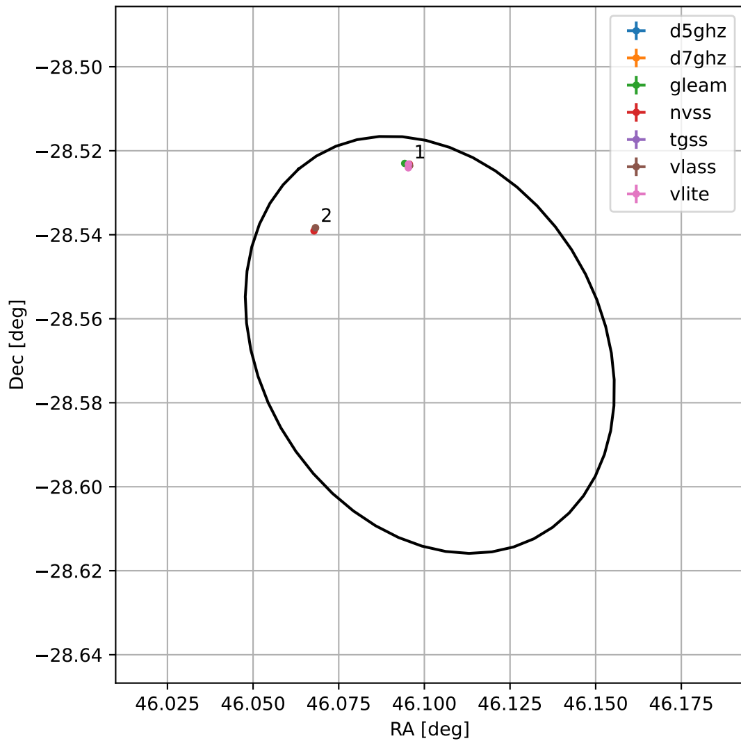
4FGL J0304.4-2833
