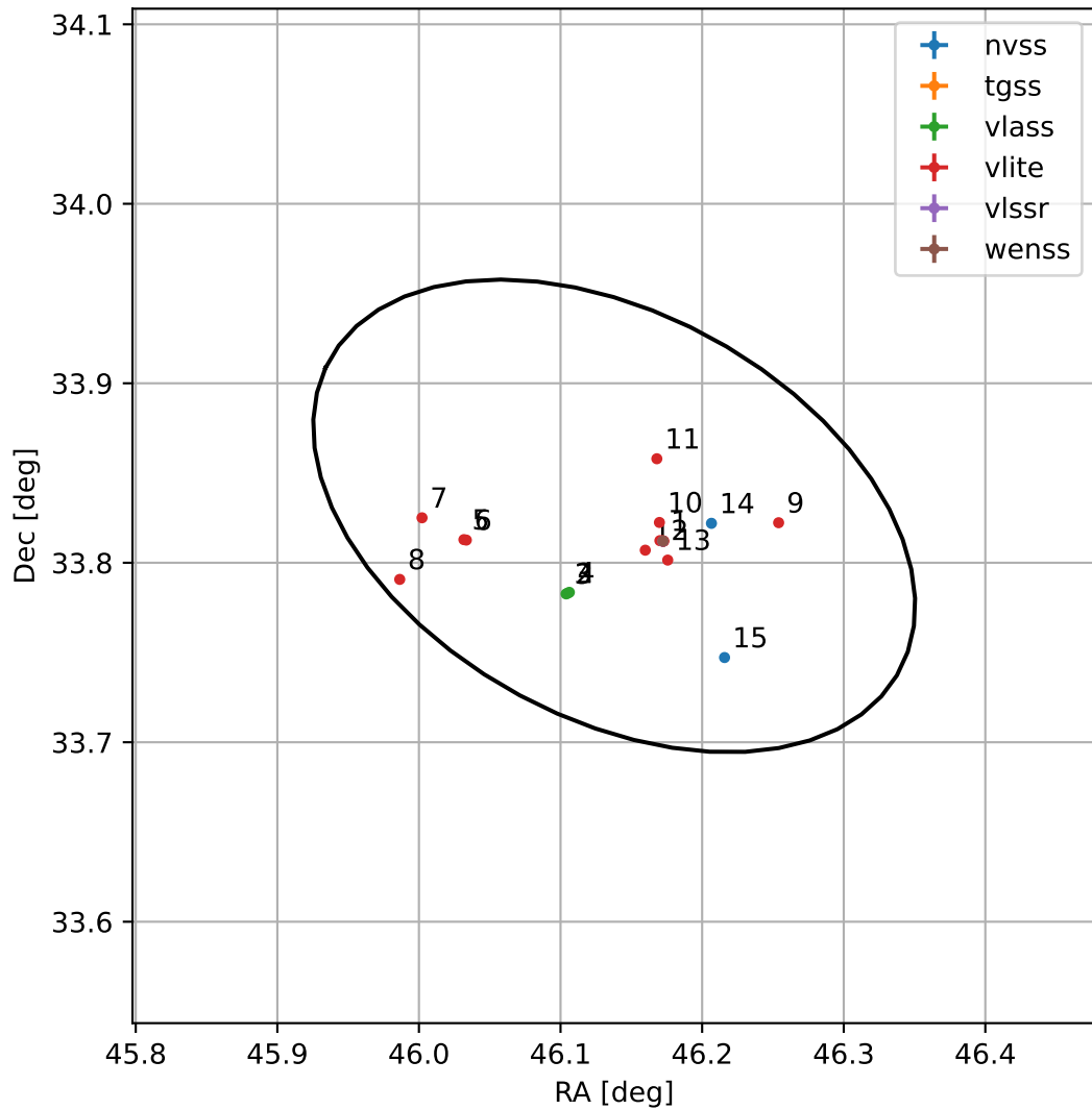
4FGL J0304.5+3349
