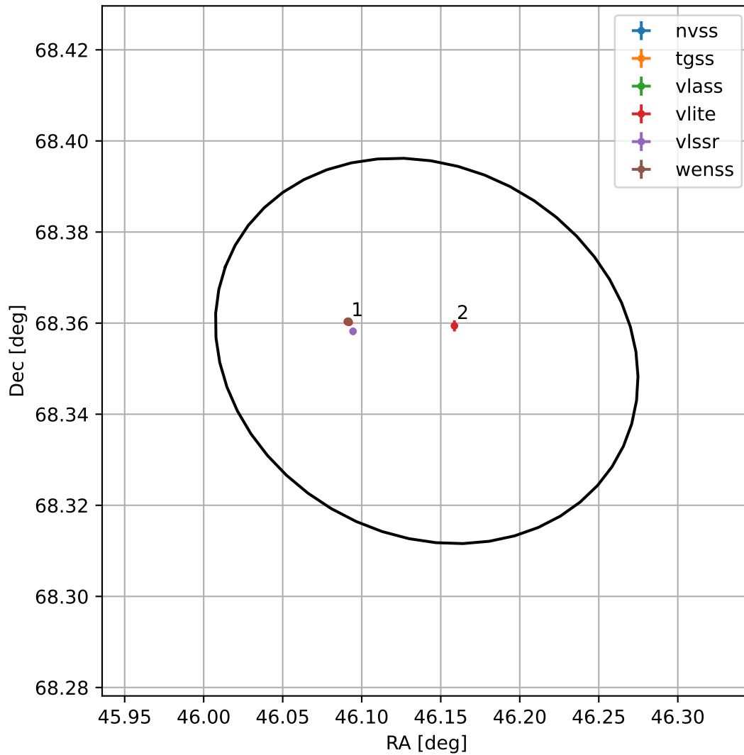
4FGL J0304.5+6821
