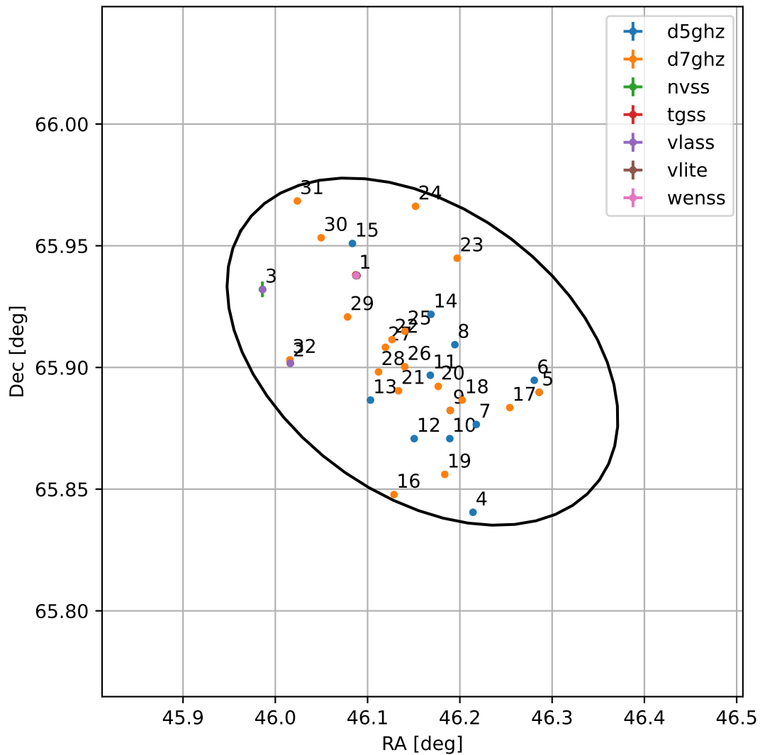
4FGL J0304.6+6554
