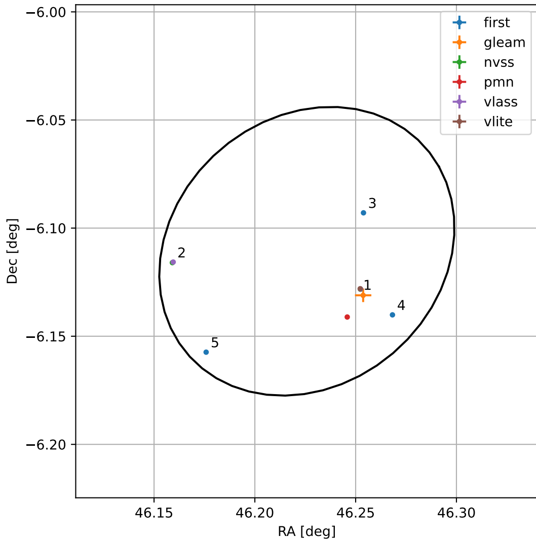
4FGL J0304.9-0606
