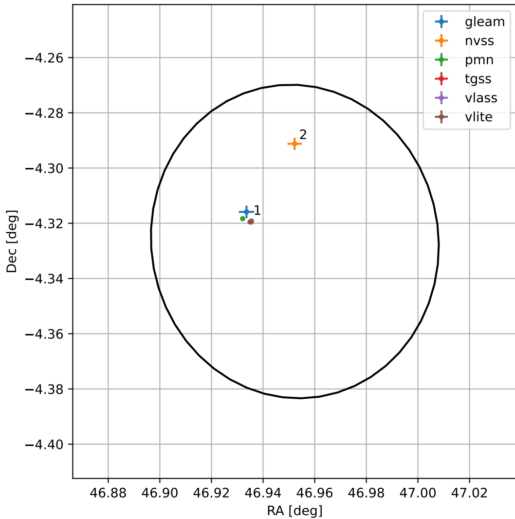
4FGL J0307.8-0419
